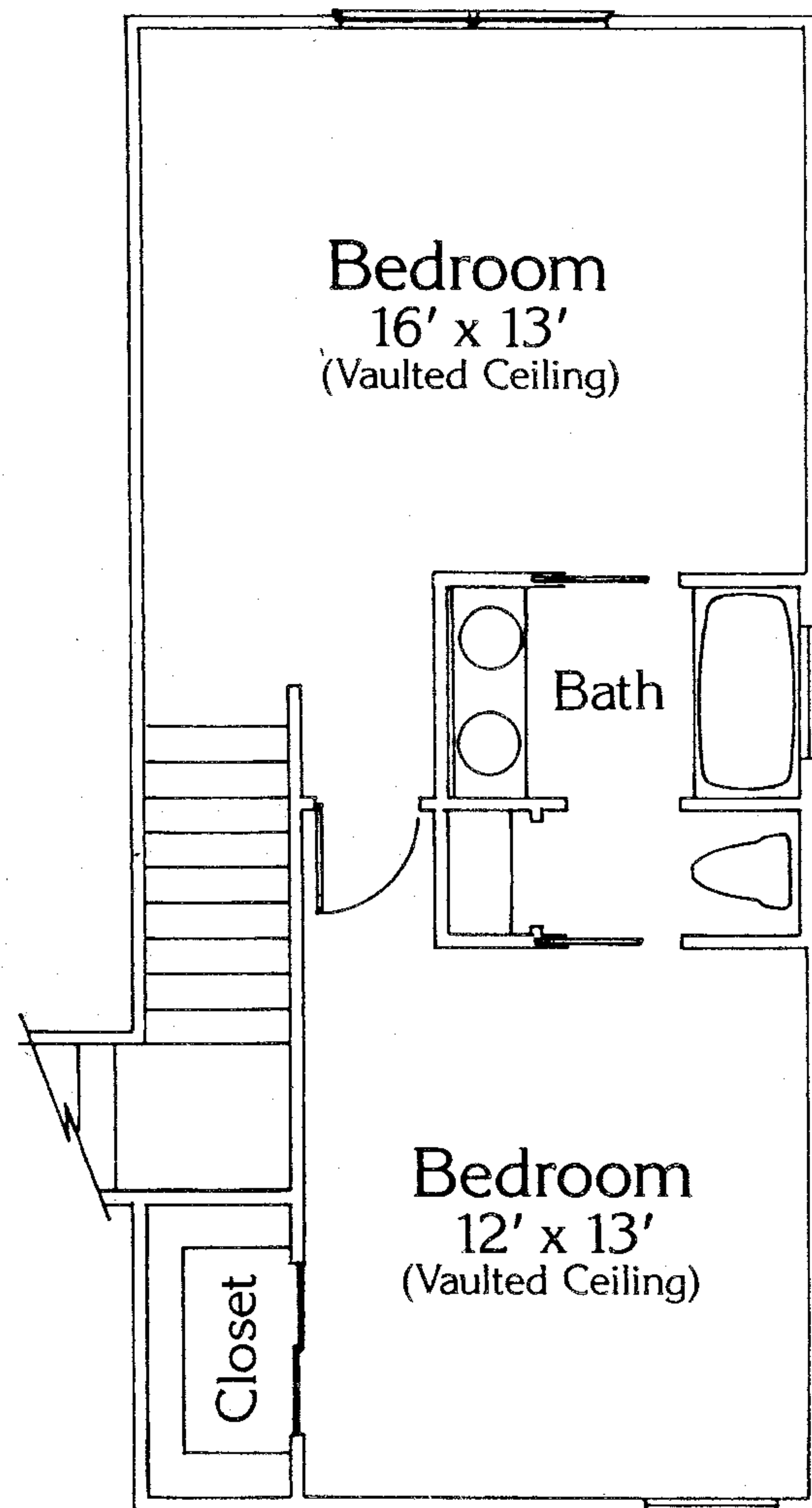
Second Floor
