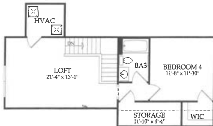
Loft w/ Bedroom and Bath
