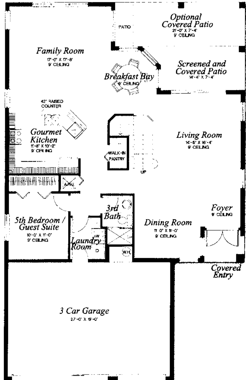
FIRST FLOOR
