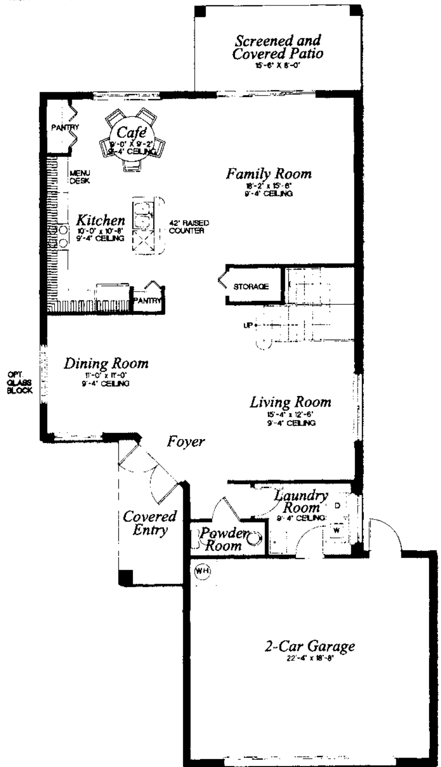
FIRST FLOOR
