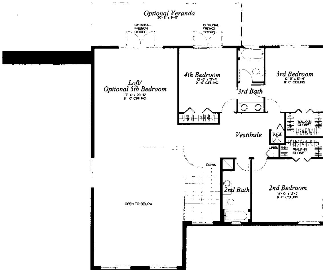
SECOND FLOOR
