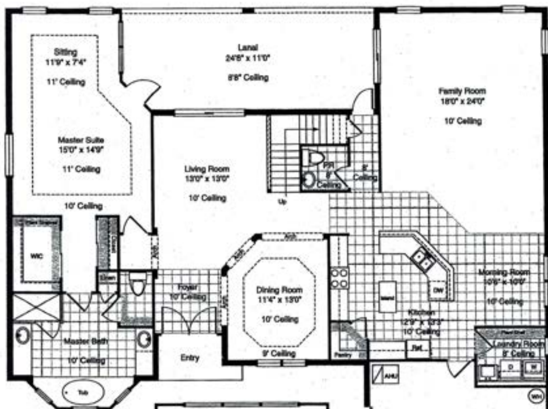
First Floor
