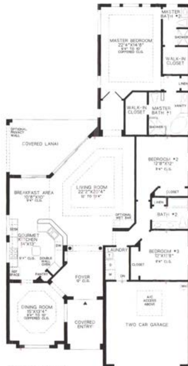
FLOOR PLAN
