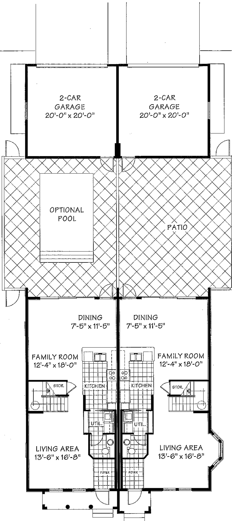
FIRST FLOOR
