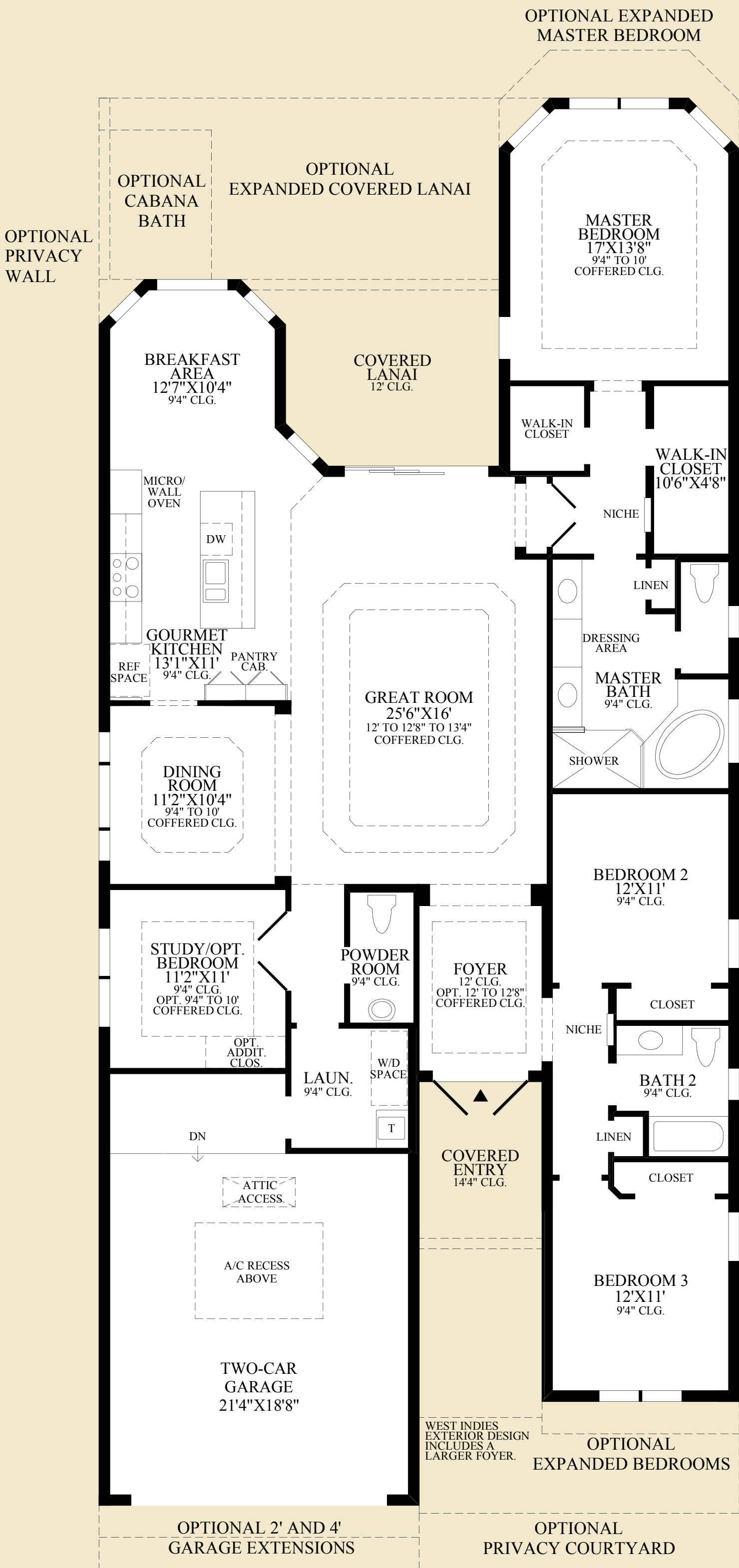
Floor Plan CARIBBEAN EXTERIOR DESIGN SHOWN
